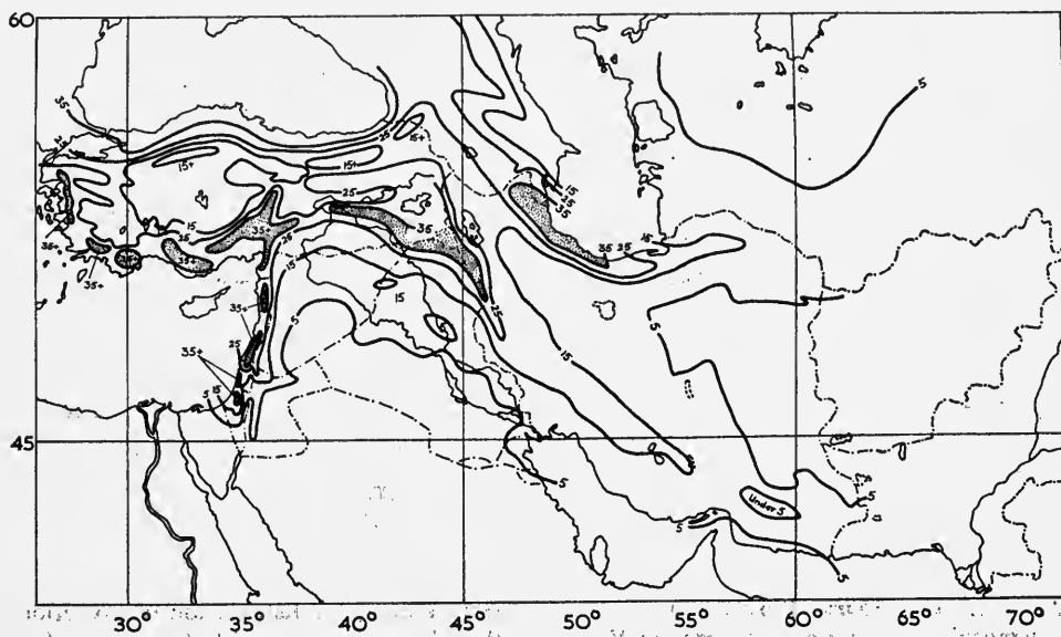
FIG. 21. Isohyets (mean annual rainfall in inches) for Middle East (various sources).
